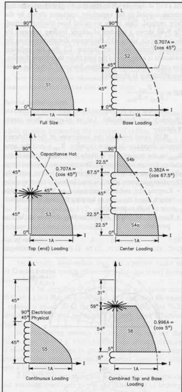
Fig 9-40—Short loaded verticals with their current distribution. The radiation resistance is proportional to the area under the current-distribution curve. The efficiency is also proportional to the radiation resistance. See text for details.
