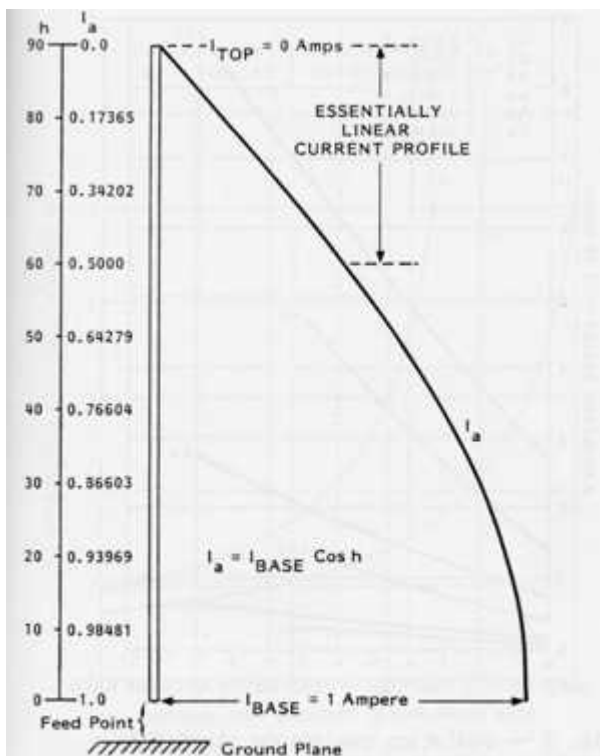
Fig. 1 — Relative current profile in a vertical antenna of height h equal to 90 electrical degrees.
