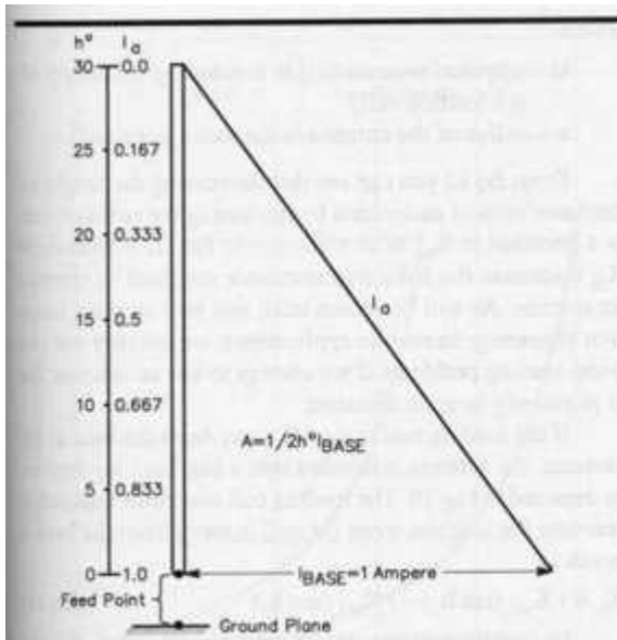
Fig 9—Relative current distribution on a base-loaded vertical antenna of height H = 30 electrical degrees (linearized). The base loading coil is not shown here.
